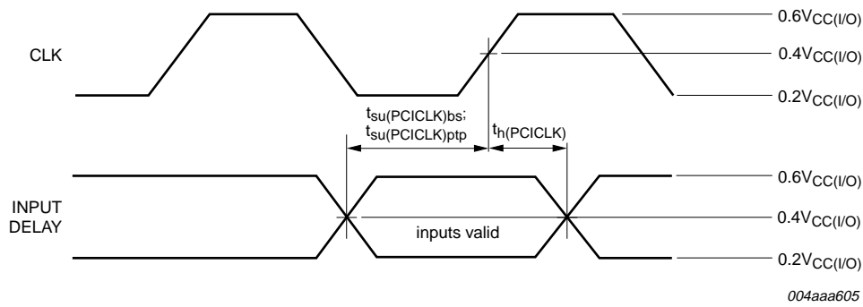
Fig 8. PCI input timing
