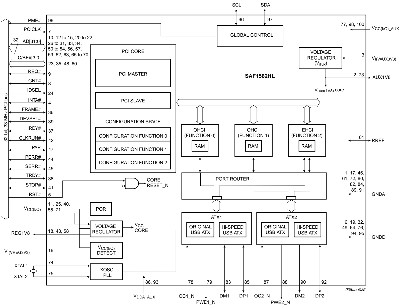
Fig 1. Block diagram of SAF1562HL
